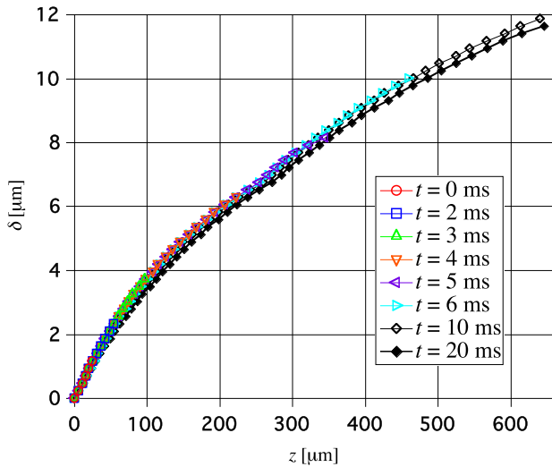
Fig. 8. Time variation of the liquid film profile.
