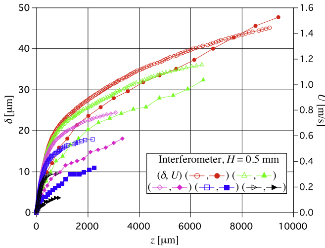
Fig. 13. Liquid film thickness and interface velocity along the flow direction, H = 0.5 mm.
