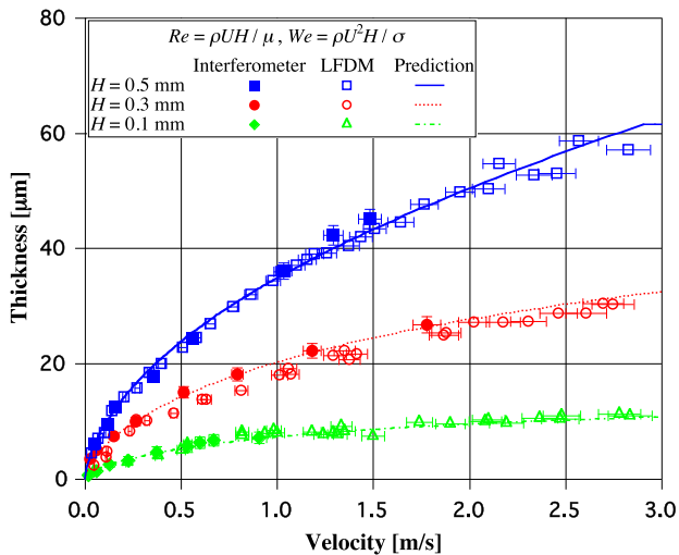
Fig. 19. Comparison between the measured liquid film thicknesses and the predicted values with Eq. (10) using hydraulic diameter as the characteristic length for Re and We .
