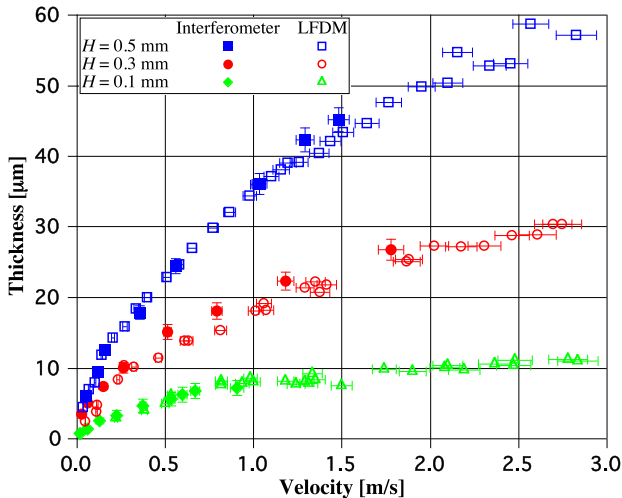
Fig. 14. Liquid film thicknesses measured by interferometer and LFD versus interface velocities.
