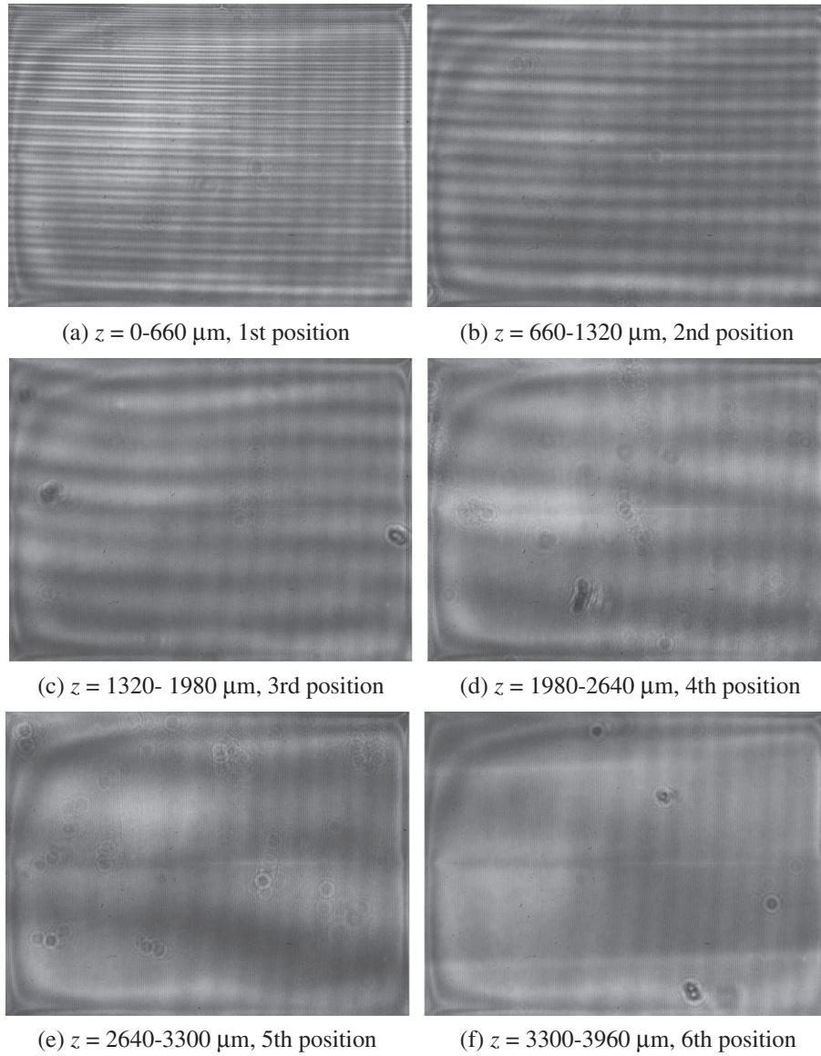
Fig. 9. Captured fringe pattern images along the flow direction: (a) z = 0\text{--}660\ \mu\text{m} , 1st position; (b) z = 660\text{--}1320\ \mu\text{m} , 2nd position; (c) z = 1320\text{--}1980\ \mu\text{m} , 3rd position; (d) z = 1980\text{--}2640\ \mu\text{m} , 4th position; (e) z = 2640\text{--}3300\ \mu\text{m} , 5th position; and (f) z = 3300\text{--}3960\ \mu\text{m} , 6th position.
