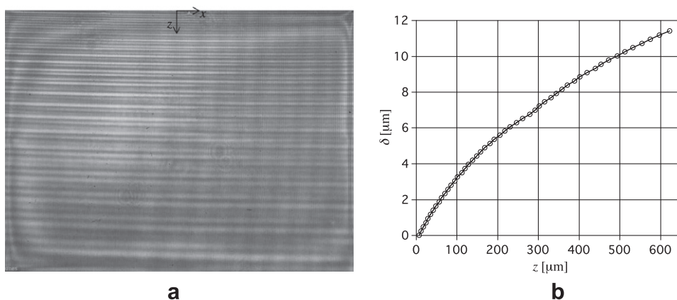
Fig. 4. Profile of liquid film thickness along the flow direction ( z -axis): (a) captured fringe pattern image and (b) calculated liquid film thickness from the fringe pattern image.
