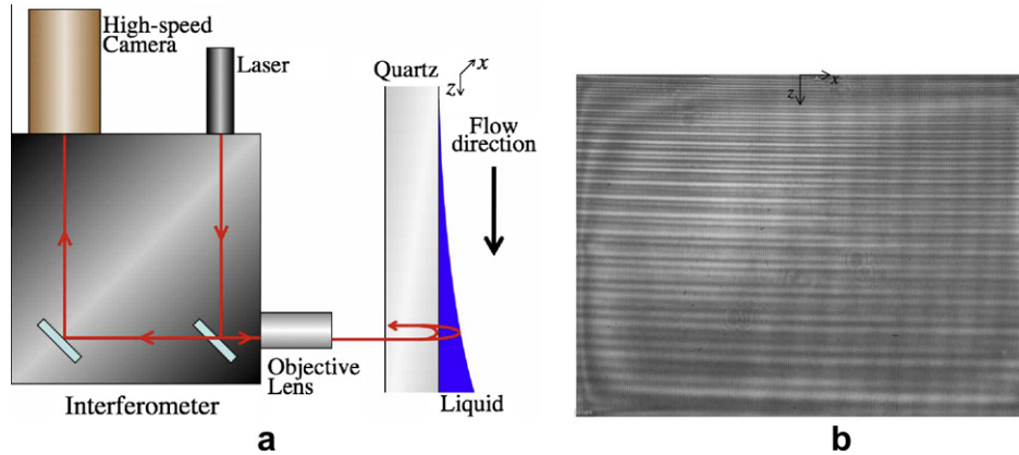
Fig. 3. Principle of interferometer: (a) schematic diagram and (b) example of fringe pattern image.
