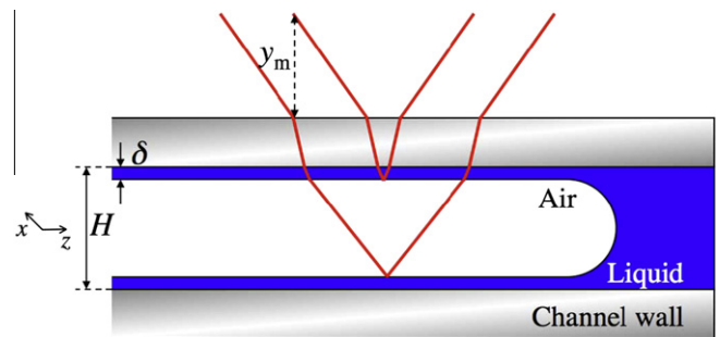
Fig. 11. Laser paths in a micro parallel channel.
