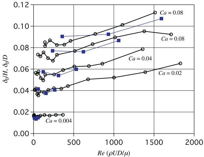
Fig. 17. Dimensionless liquid film thickness versus Reynolds number at fixed capillary numbers.
