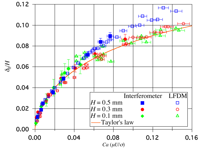
Fig. 15. Dimensionless liquid film thicknesses \delta_0/H versus capillary number Ca = \mu U/\sigma .
