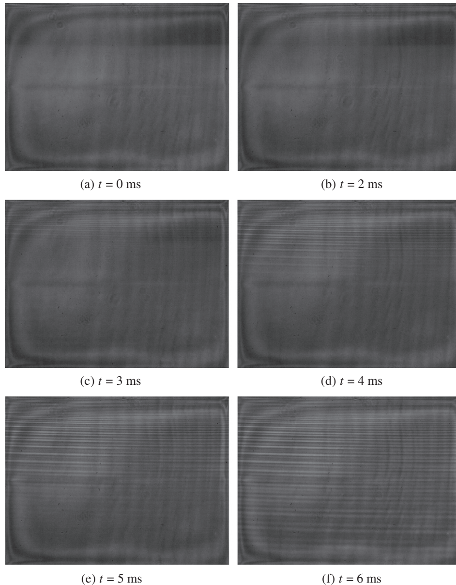
Fig. 7. Time variation of fringe pattern image at first position at: (a) t = 0 ms, (b) t = 2 ms, (c) t = 3 ms, (d) t = 4 ms, (e) t = 5 ms, (f) t = 6 ms, (g) t = 8 ms, (h) t = 10 ms, (i) t = 15 ms, and (j) t = 20 ms.
