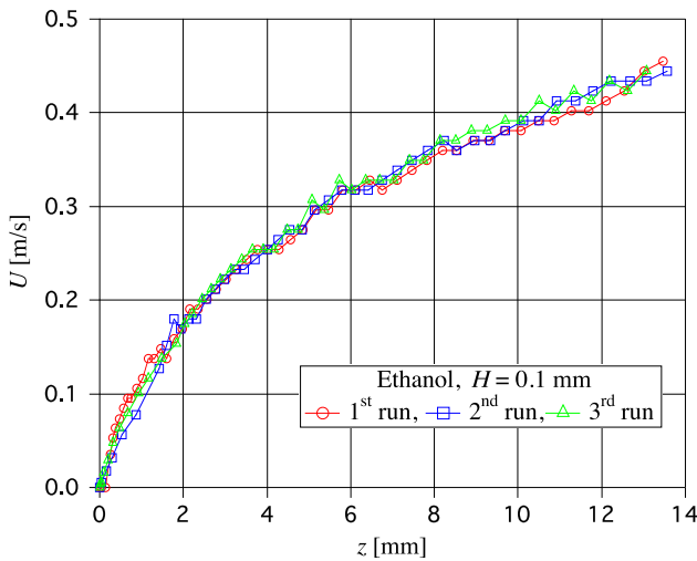
Fig. 6. Measured velocity variations along the flow direction.
