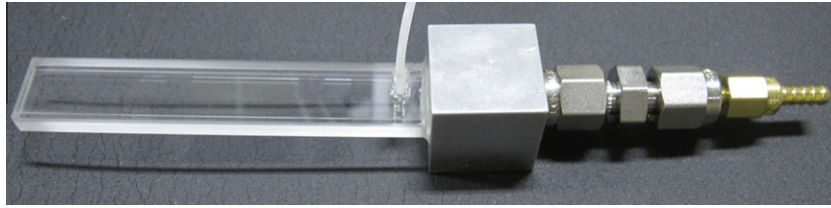
Fig. 2. Aluminum block connected to the high aspect ratio rectangular channel.
