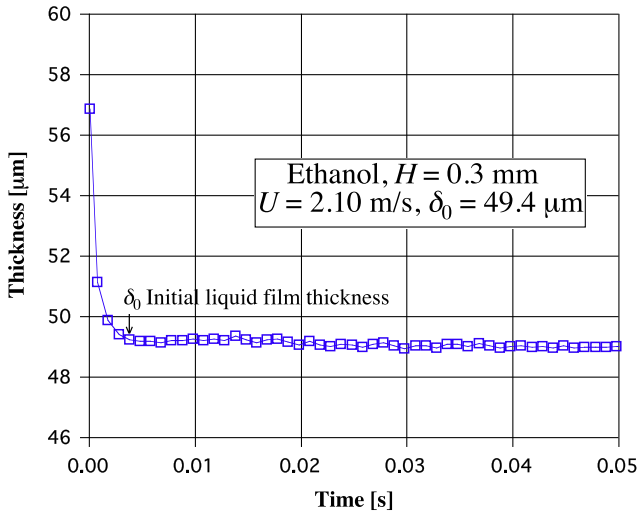
Fig. 12. Time variation of liquid film thickness measured by laser focus displacement meter.
